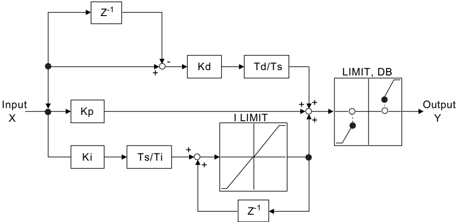
Block Diagram
